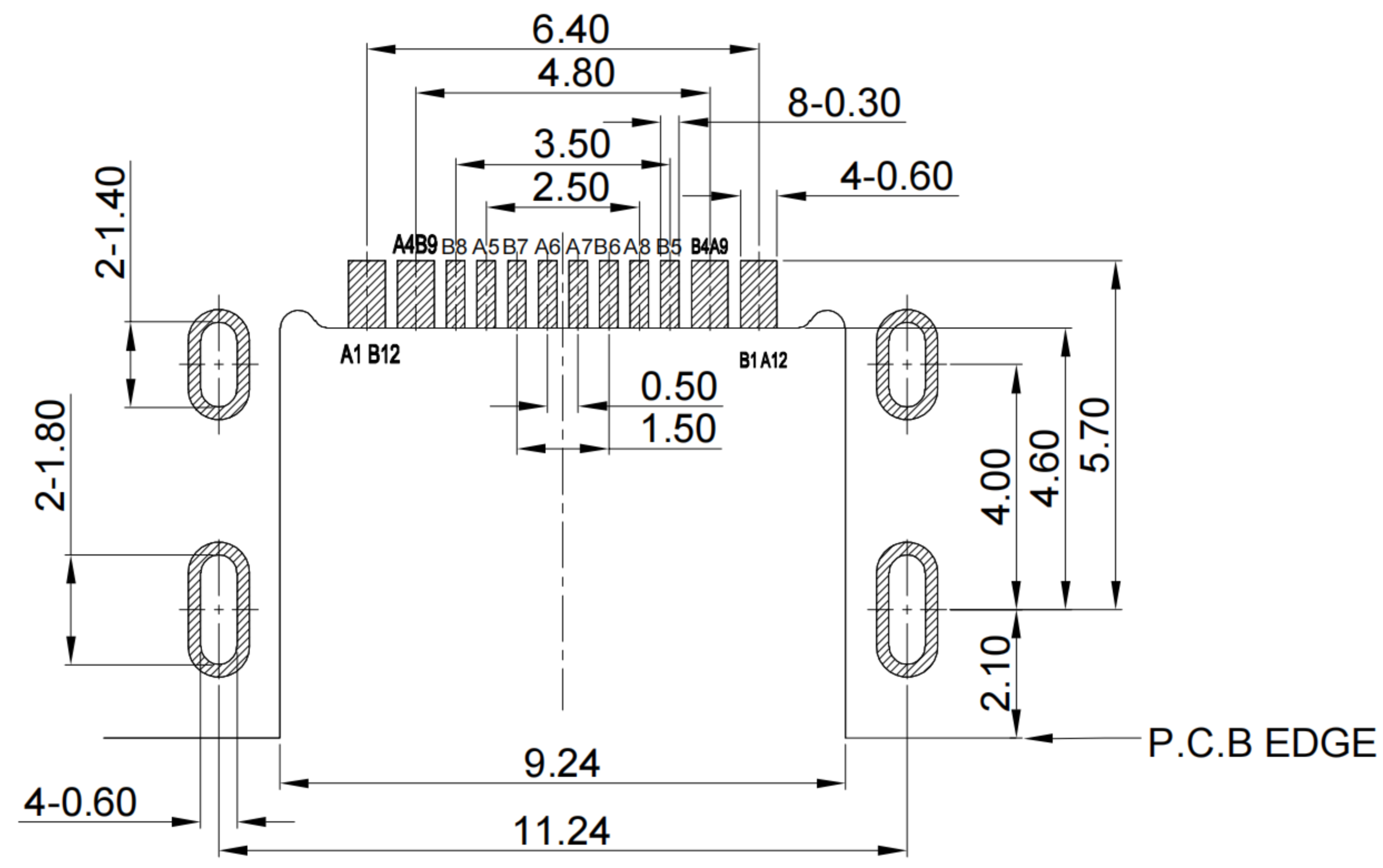
RECOMMENDED PCB LAYOUT TOLERANCE:±0.05
