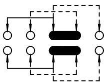
SCHEMATIC (SHORTING)
