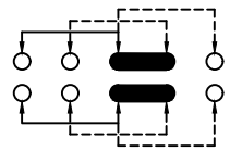
SCHMATIC (SHORTING)
