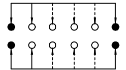
SCHEMATIC (NON-SHORTING)
