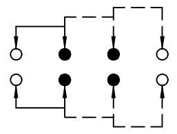
SCHMATIC (NON-SHORTING)
